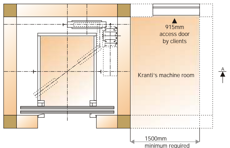
Plan of liftwell and Kranti's machine room for center opening door lift.
