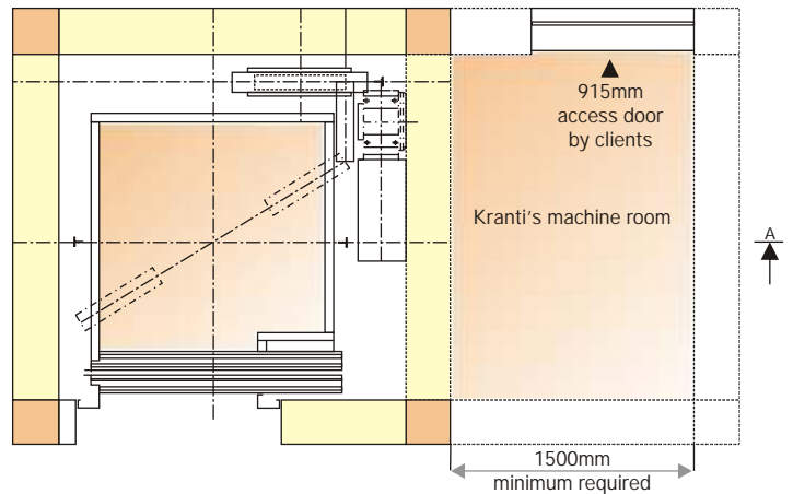
Plan of liftwell and Kranti's machine room for side opening telescopic door lift.
